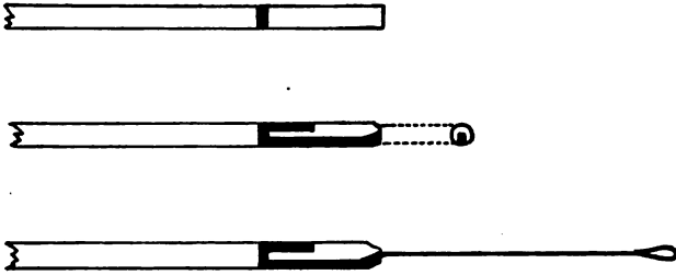
FIG. 64.—Platinum rod in aluminium handle—method of mounting.
